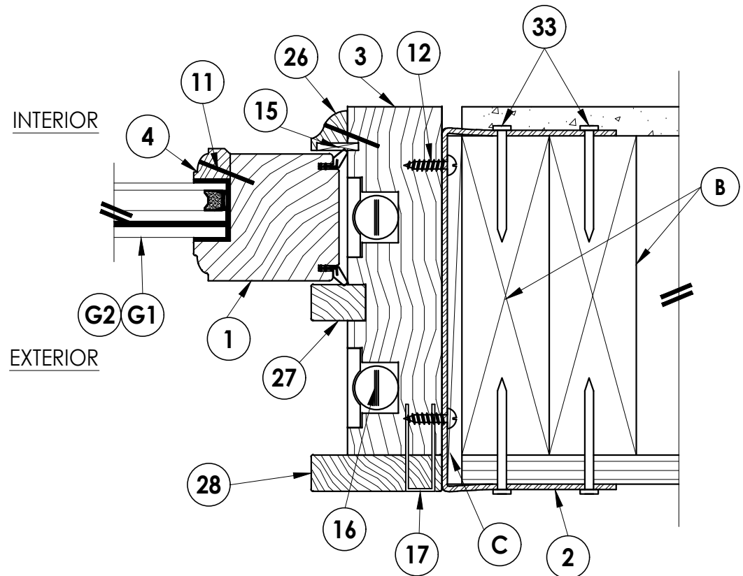
4/4 HORIZONTAL CROSS SECTION
