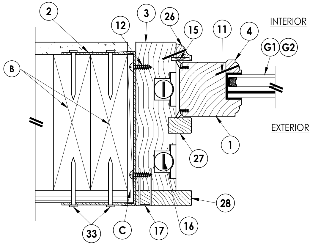
3/4 HORIZONTAL CROSS SECTION
