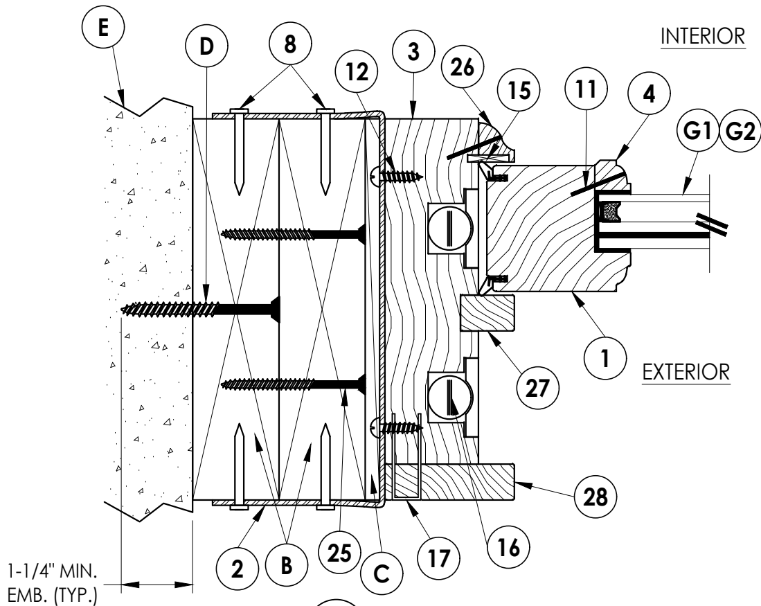
3 2 HORIZONTAL CROSS SECTION
