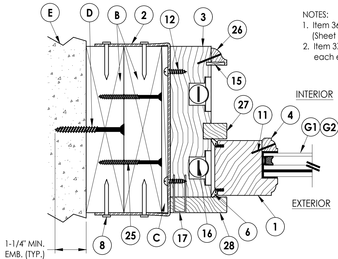
1 2 HORIZONTAL CROSS SECTION
